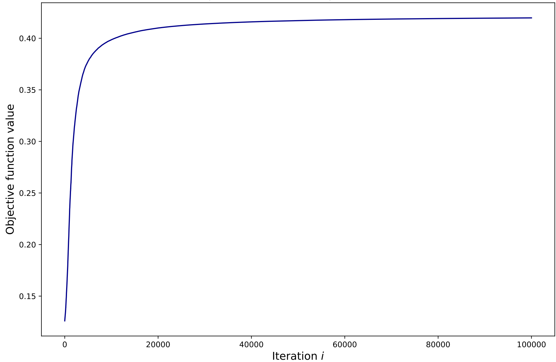
Objective function value per iteration i
