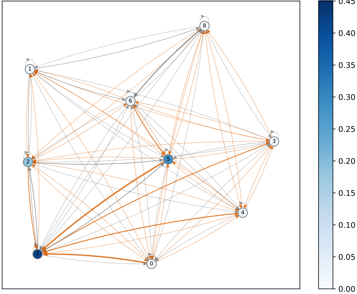
The final network with nodes coloured by their stationary distribution value
